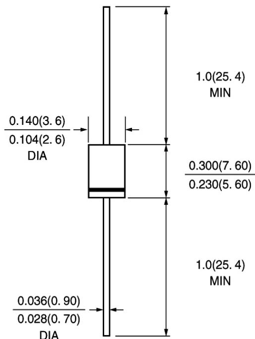
DO-15\DO-204AC
