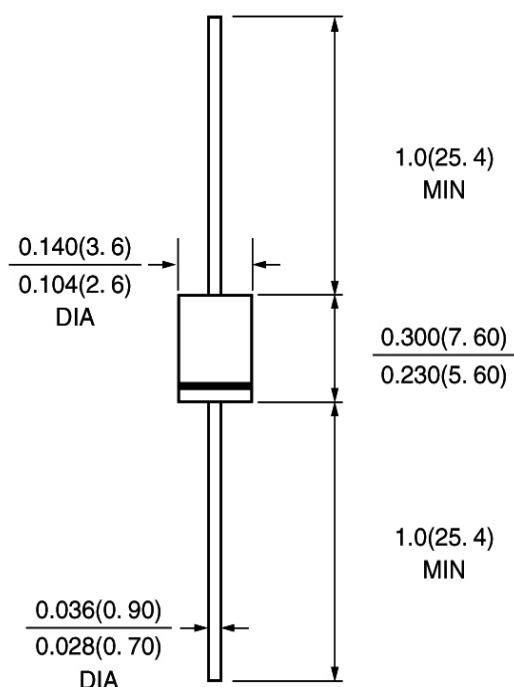
DO-15\DO-204AC
