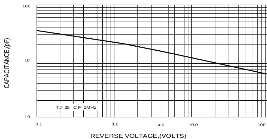
FIG.4-TYPICAL JUNCTION CAPACITANCE
