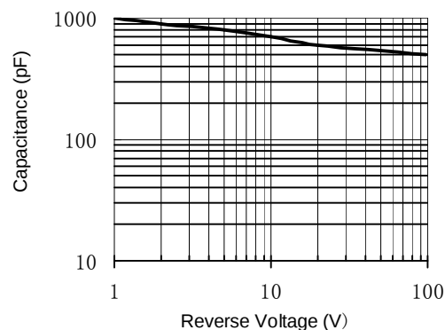
The crunode capacitance curve
