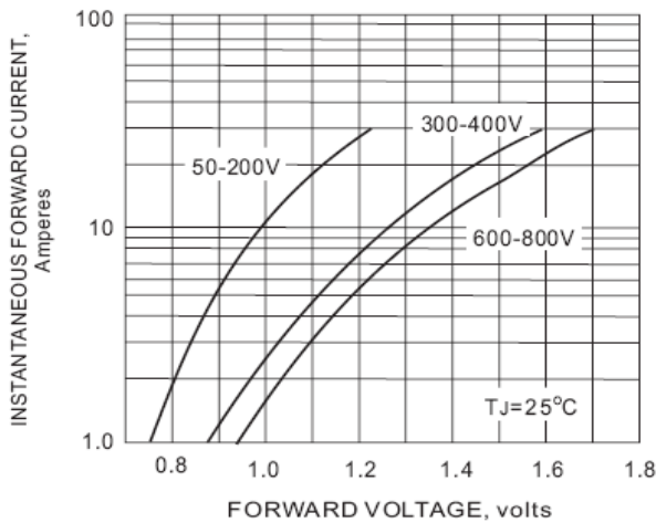
Fig.3 FORWARD CHARACTERISTICS
